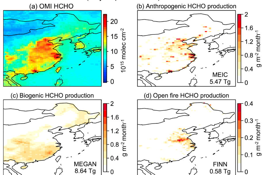
Figure 2. Mean HCHO over China in May–September 2005–2016 and its sources as estimated from bottom-up emission inventories of nonmethane VOCs. (a) HCHO columns from the OMI-SAO satellite retrieval with bias correction applied (section 2). (b) Mean anthropogenic production rate derived from MEIC VOC emissions with 1-day HCHO yields. (c) Same as (b) but for biogenic emissions from MEGAN v2.1 driven by 2005 MERRA2 meteorology. (d) Same as (b) but for open fires from FINN. Note the lower scale for open fire emissions. The HCHO 1-day yields from oxidation of different VOC species are from Chan Miller et al. (2016), as given in Table S1. The May–September total HCHO production amounts during 2005–2016 from each source type in eastern China (east of 103°E, covering the map domain) are shown inset. HCHO = formaldehyde; VOC = volatile organic compound; MEIC = Multi-resolution Emission Inventory for China; FINN = Fire INventory from NCAR.
