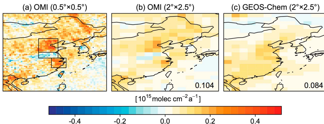
Figure 3. The 2005–2016 trends of formaldehyde (HCHO) columns over China. Values are fitted linear trends for May–September 5-month averages of each year. OMI trends are corrected for temperature as described in the text. (a) Observed OMI trends on the 0.5^\circ \times 0.5^\circ grid. From top to bottom, the three rectangles delineate the North China Plain, Huai River Basin, and Yangtze River Delta. (b) Same as (a) but on a 2^\circ \times 2.5^\circ grid. (c) 2005–2016 trends simulated by GEOS-Chem at 2^\circ \times 2.5^\circ resolution with fixed biogenic sources at the 2005 level. The averaged trends in eastern China are shown inset.
